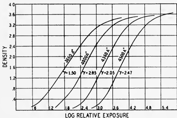
FIG. 4. Variation of gamma with wavelength for E.K. 1301 emulsion.
